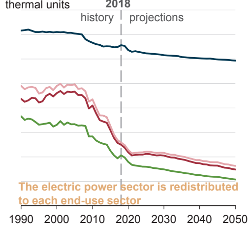
Carbon dioxide intensity by end-use sector (Reference case)
